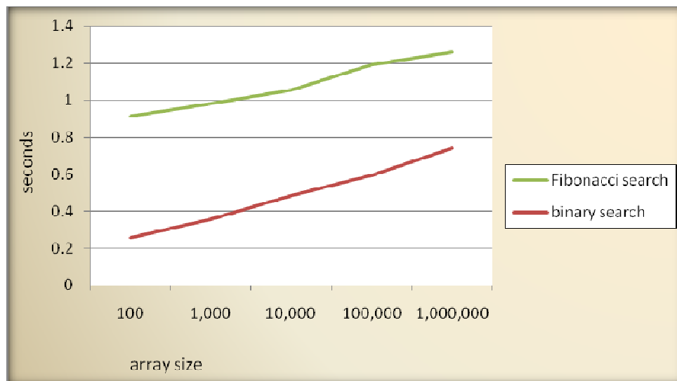
The results for 200 pseudorandom numbers, each sought for 10,000 times
