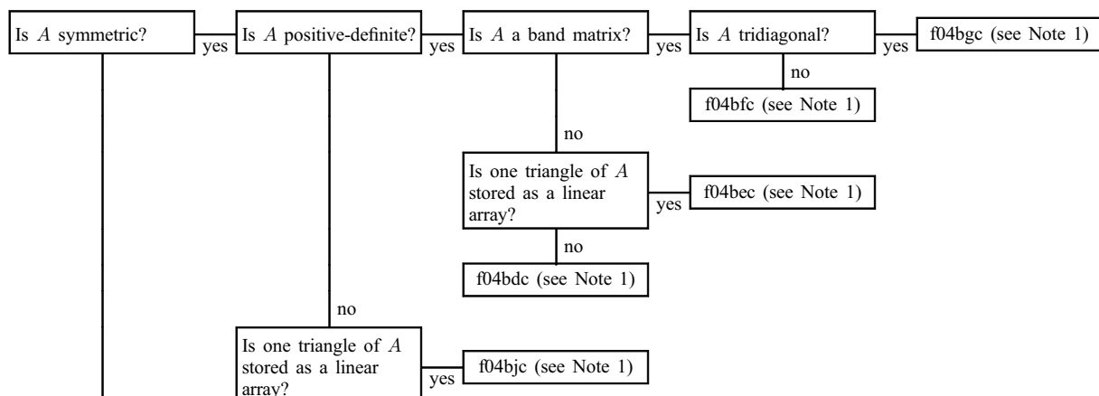
Tree 1: Black Box functions for unique solution of Ax = b (Real matrix)
