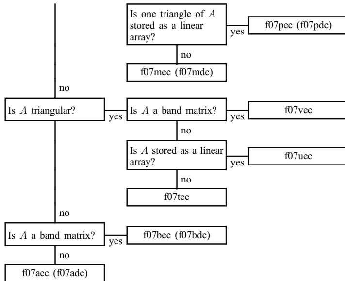
Tree 4: General purpose functions for unique solution of Ax = b (Complex matrix)
