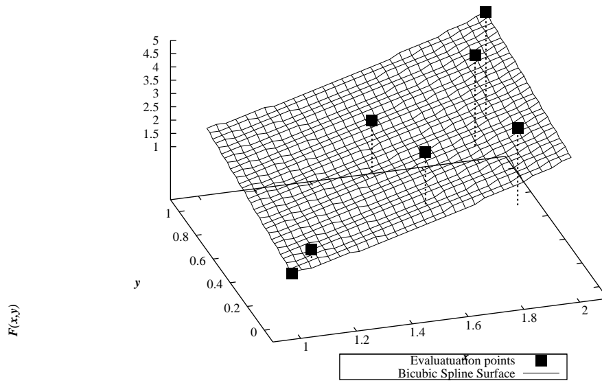
Example Program Evaluation of Least-squares Bicubic Spline Fit at Scattered Points
